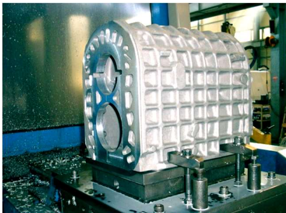
BUS TRANSMISSION CASE
